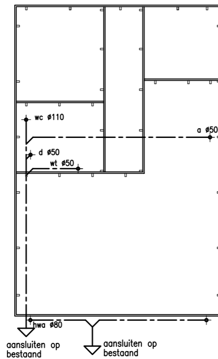
Funderingsplan-riolering
